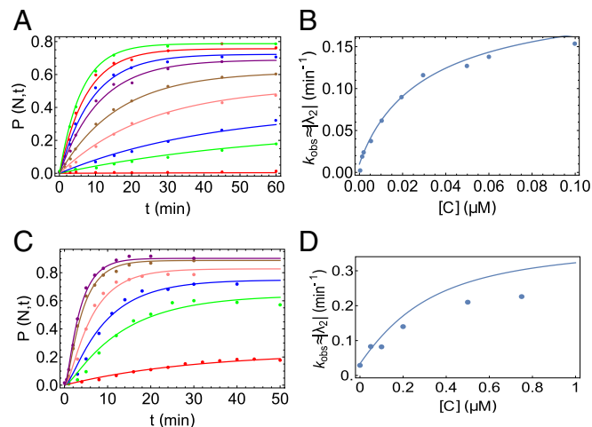
Fig. 6. Using the kinetic model to analyze GroEL-assisted folding of Rubisco and MDH. (A) Quantitative fits of a time-dependent increase of folded Rubisco at various GroEL concentrations and 1 \text{ mM} ATP using our kinetic model (data taken from ref. 17). Note that the y axis was converted to a fraction between 0 and 1 by dividing Rubisco concentrations by 50 \text{ nM} , which was the starting concentration of acid-denatured protein in ref. 17. The concentrations of GroEL are (from bottom to top) 0, 1, 2, 5, 10, 20, 30, 50, and 100 \text{ nM} . A single set of parameters, listed in Table S2, fits all of the curves. The dependence in the steady-state values of P(N, t) (t \approx 60 \text{ min}) is an indication of the departure from equilibrium. In all cases, P(N, t) (t \approx 60 \text{ min}) is less than the equilibrium value. (B) Dependence of the rate k_{obs} as a function of native MDH at various GroEL concentrations and 500 \mu\text{M} ATP. Initial concentration of denatured MDH (dMDH) was 0.5 \mu\text{M} . Concentrations of GroEL are (from bottom to top) 0, 0.05, 0.1, 0.2, 0.5, and 0.75 \mu\text{M} . (D) Dependence of the rate k_{obs} as a function of GroEL concentration for folding of MDH. In all panels the dots represent data from experiments, while the curves represent theoretical predictions.
