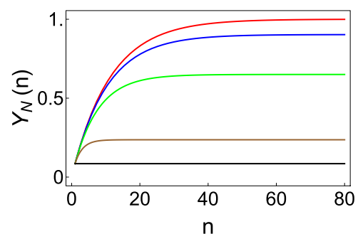
Fig. 3. Generalized IAM for proteins and RNA, showing the effect of varying \kappa on the yield of the N state. Shown is the plot of the yield, Y_N(n) (see Eq. 7), as a function of number of cycles n . The native fraction in the limit of large n therefore depends on \kappa , the efficiency of chaperone recognition of the N state: \kappa = 0 (red), \kappa = 0.01 (blue), \kappa = 0.05 (green), \kappa = 0.3 (brown), and \kappa = 1.0 (black).
