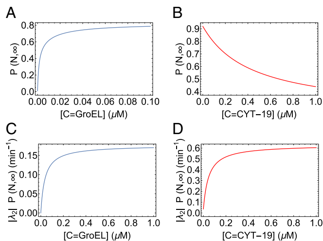
Fig. 7. Maximization of the finite-time yield by iterative annealing. (A and B) Steady-state yield of the N state of Rubisco (A) and ribozyme (B), as functions of chaperone concentration. (C and D) Plots of \Delta_{NE} = |\lambda_2|P(N, \infty) for protein (C) and ribozyme (D), as functions of chaperone concentration. The curves in A and C were obtained using the best fit parameters for the GroEL–Rubisco system, given in Table S2. The curves in B and D have been produced using the best fit parameters for the mutant P5a ribozyme, given in Table S1. For all of the curves, the ATP concentration [T] was set to 1 mM. The qualitative results do not change for other concentrations of ATP.
